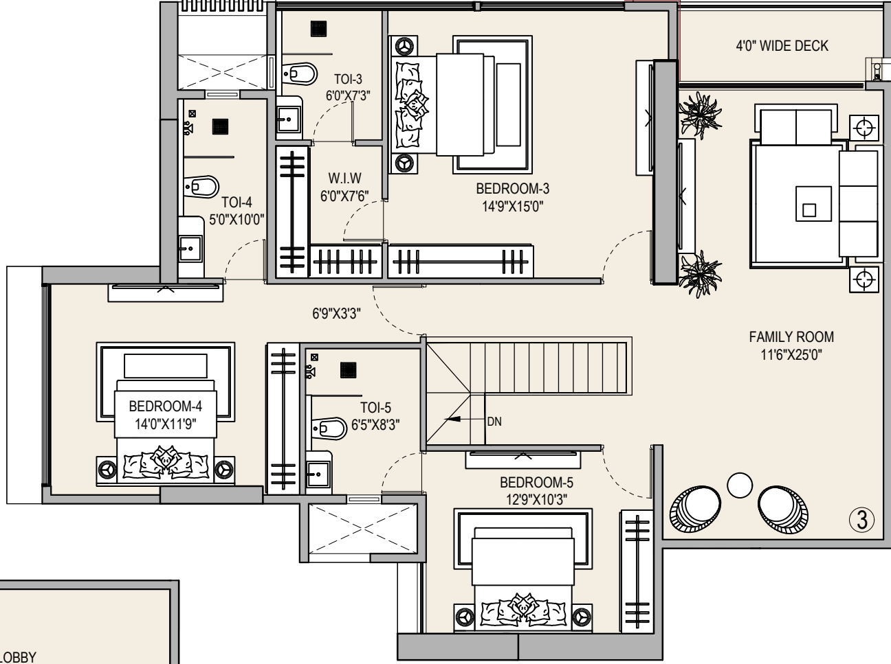
2203 - UPPER LEVEL
