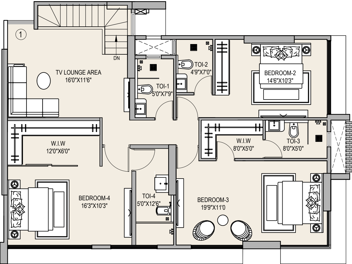
2201 - UPPER LEVEL
